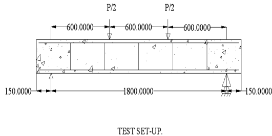
Fig. 2 Shear Test Configuration
