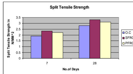
Fig. 5 Split Tensile Strength of Concrete
