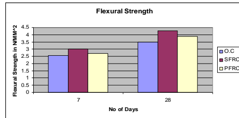
Fig. 4 Flexural strength of concrete
