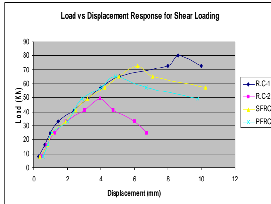
Fig. 6 Load-Displacement Response under Shear Loading
